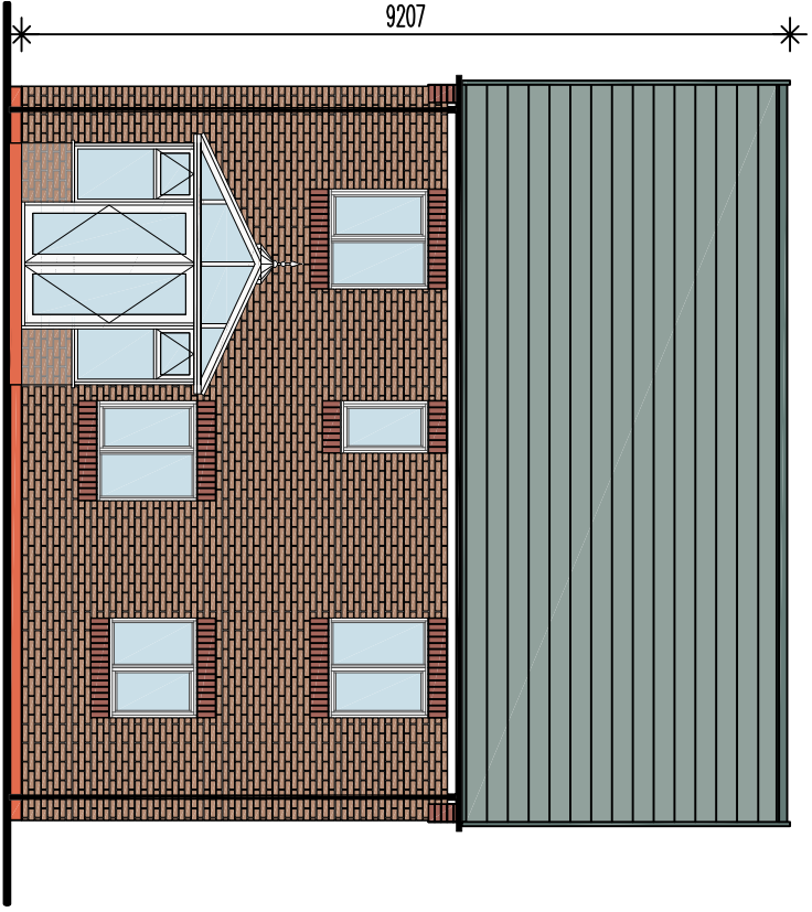
rear elevation - with conservatory option
