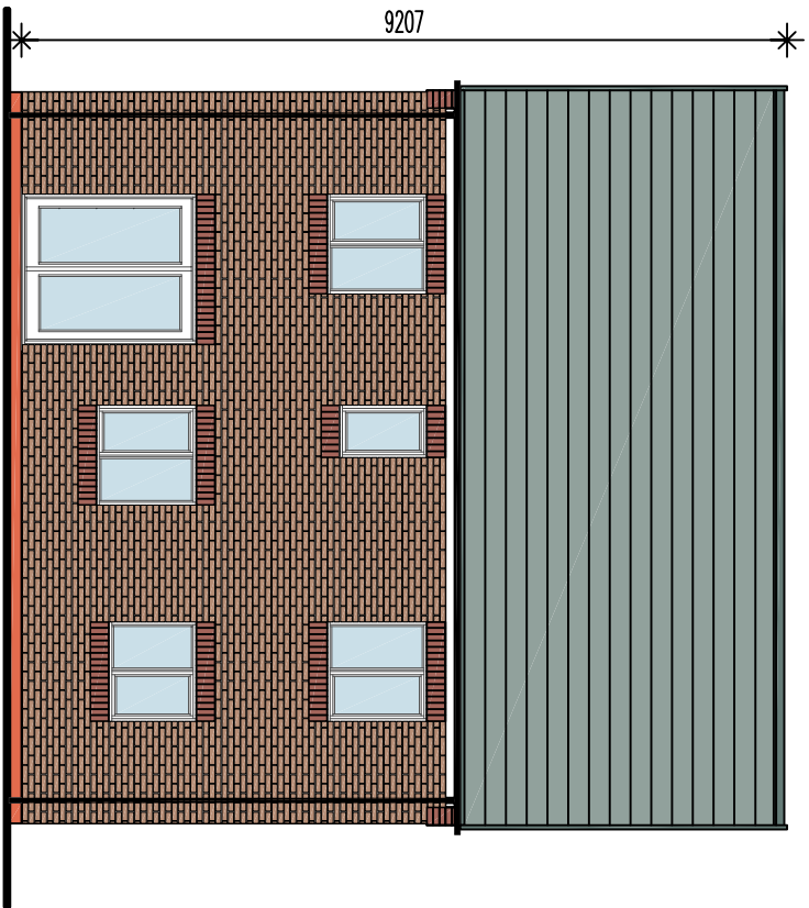
rear elevation
