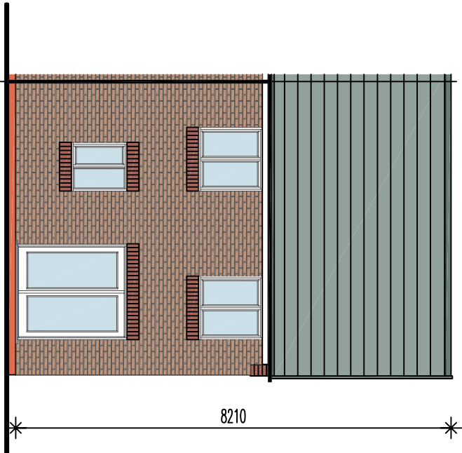
rear elevation
