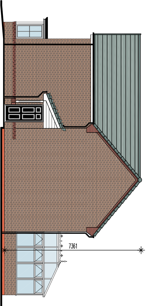
side elevation - with conservatory option
