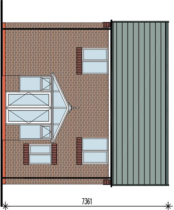
rear elevation - with conservatory option
