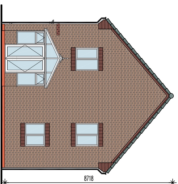
r.h. side elevation - with conservatory option
