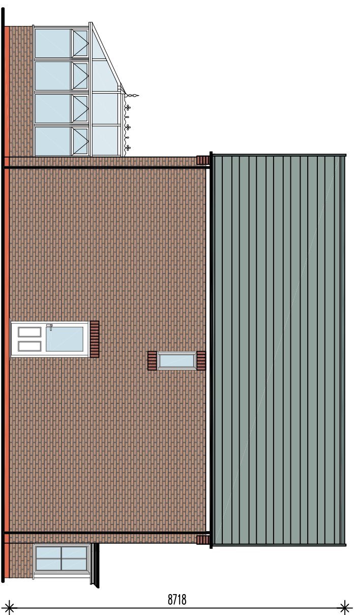
rear elevation - with conservatory option
