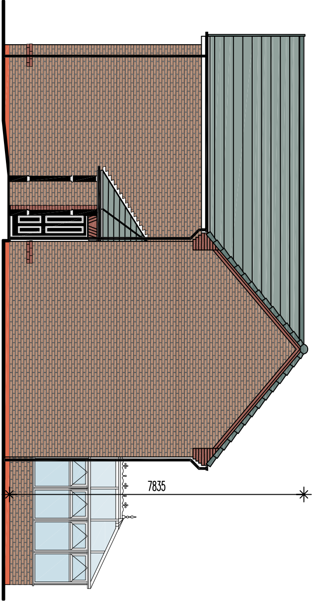
side elevation - with conservatory option
