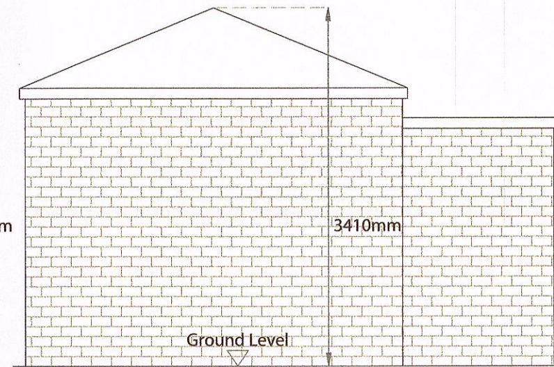
REAR ELEVATION
