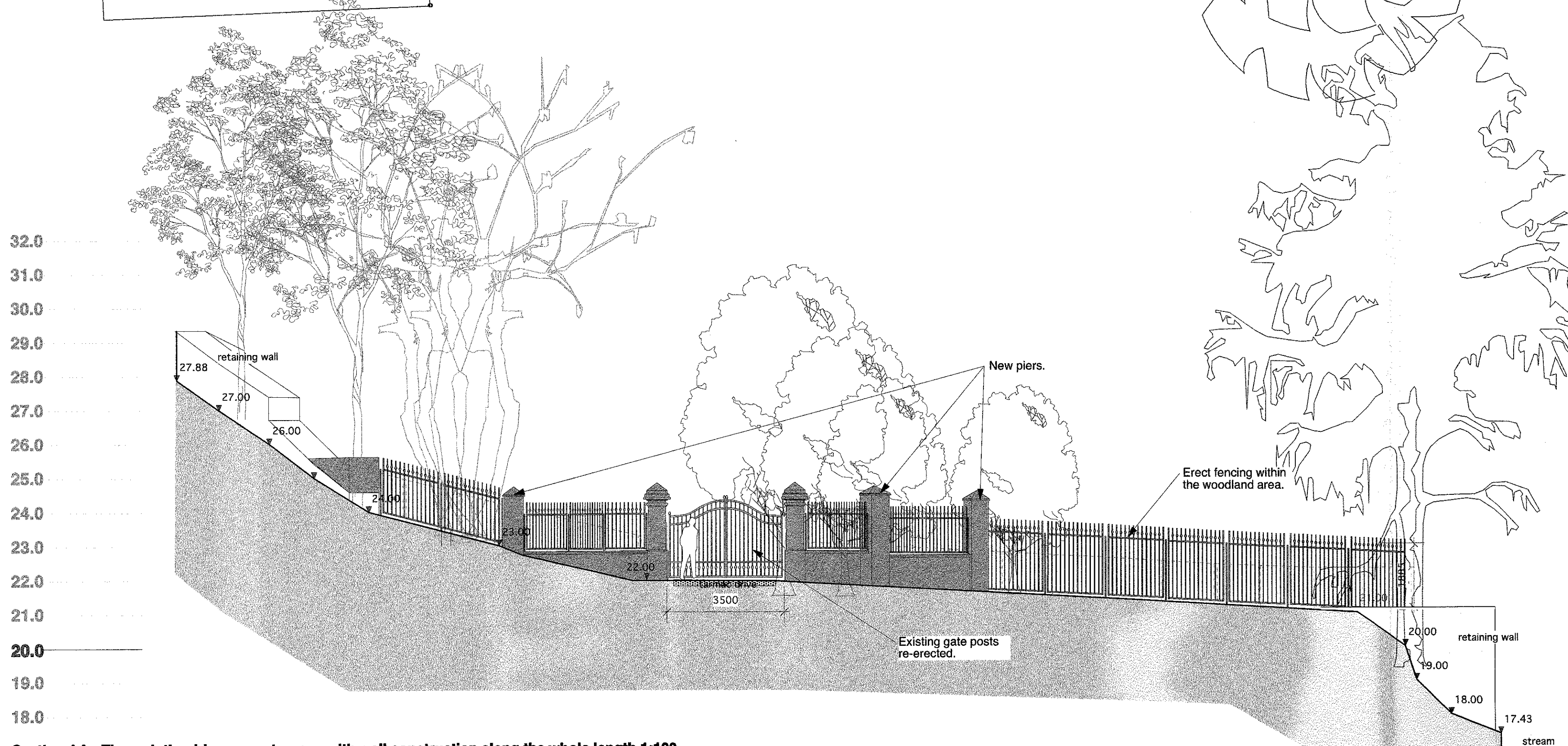
Section AA - Through the driveway entrance - with wall construction along the whole length 1:100
