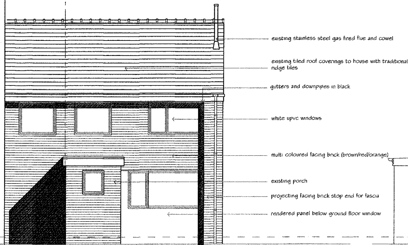
FRONT ELEVATION
