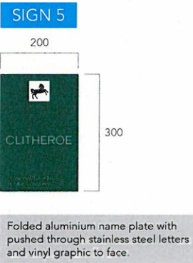
SIGN ELEVATIONS
