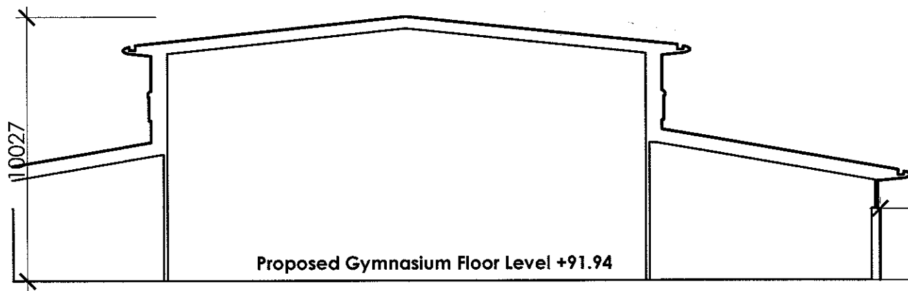
SECTION A-A: PROPOSED DESIGN SECTION IN CONTEXT - 1:200
