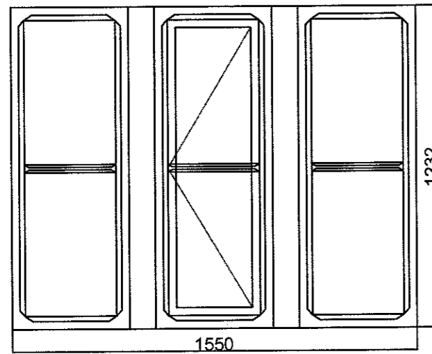
W1, 3, 7 & 8 - Existing Single Glazed with Central Opener
