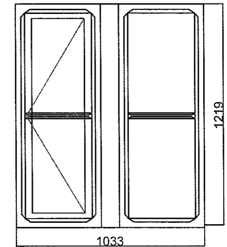
W6, 9 & 11 Single Opener
