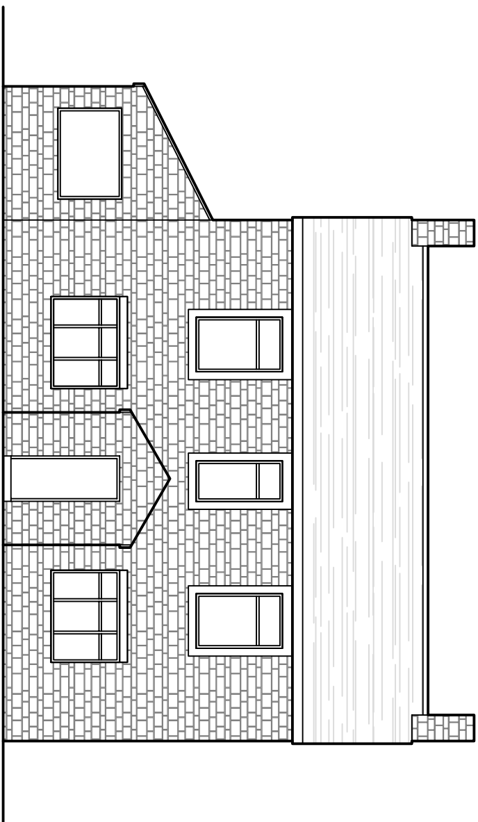
EXISTING FRONT (EAST) ELEVATION
