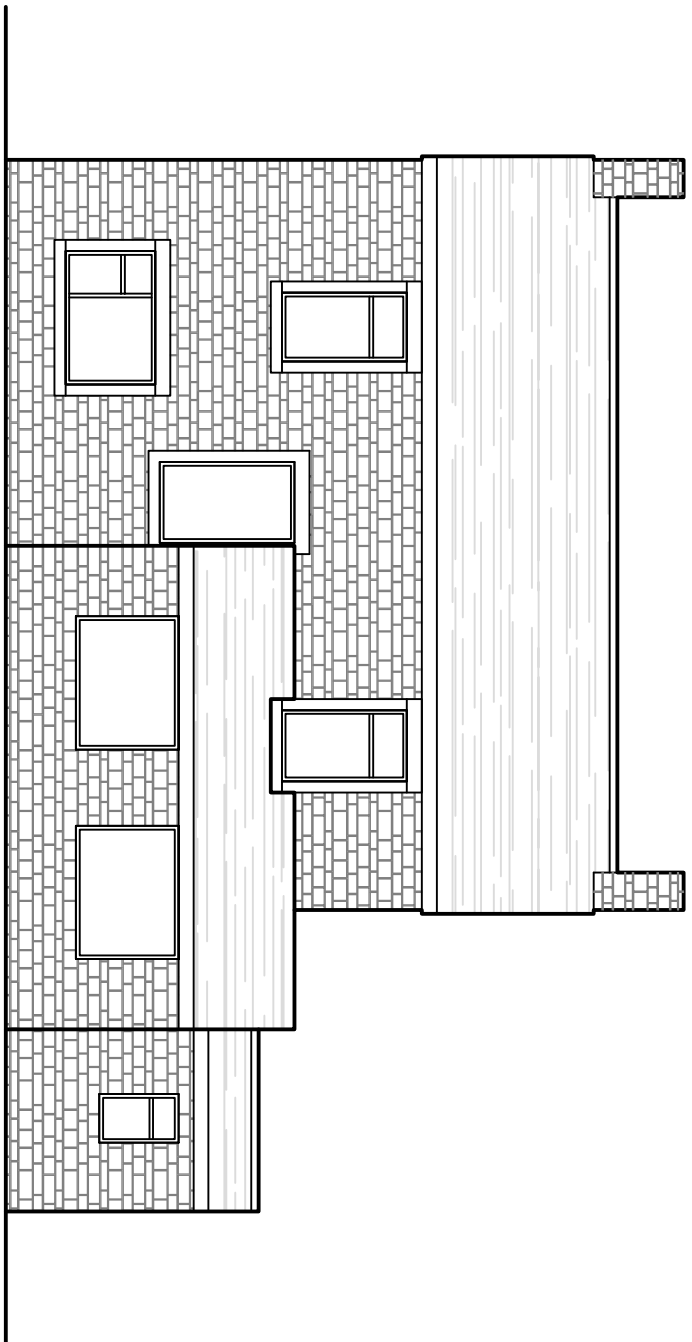
EXISTING REAR (WEST) ELEVATION
