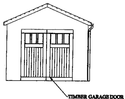
PROPOSED NORTH ELEVATION
