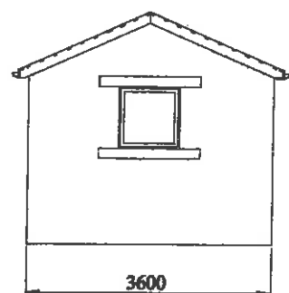
PROPOSED NORTH ELEVATION
