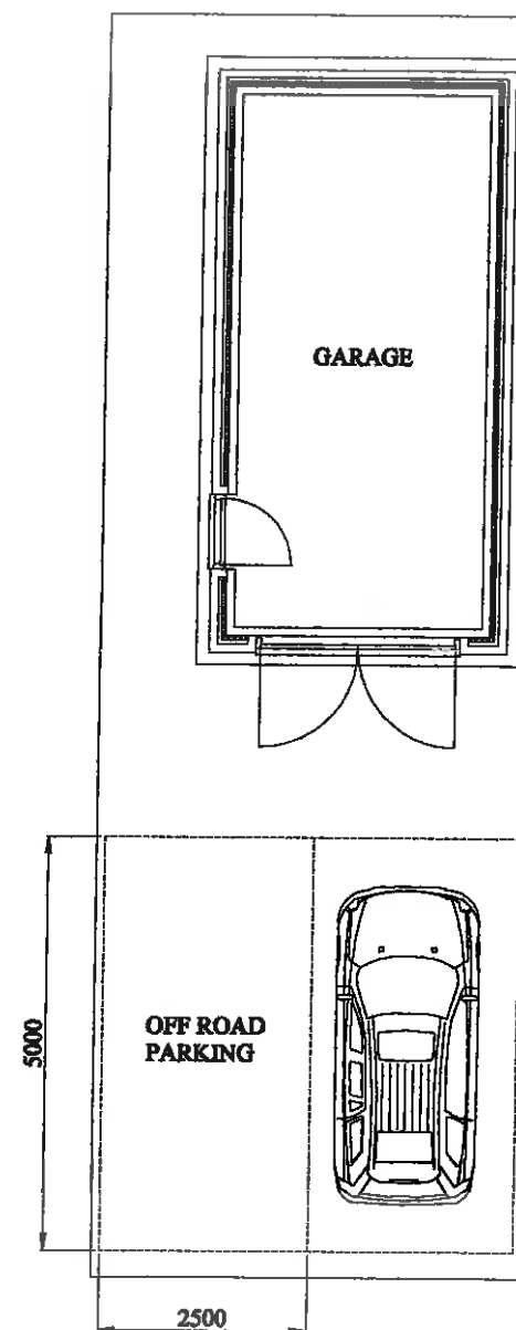
PROPOSED PLAN VIEW
