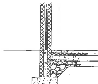
PROPOSED SECTION (1:50)
