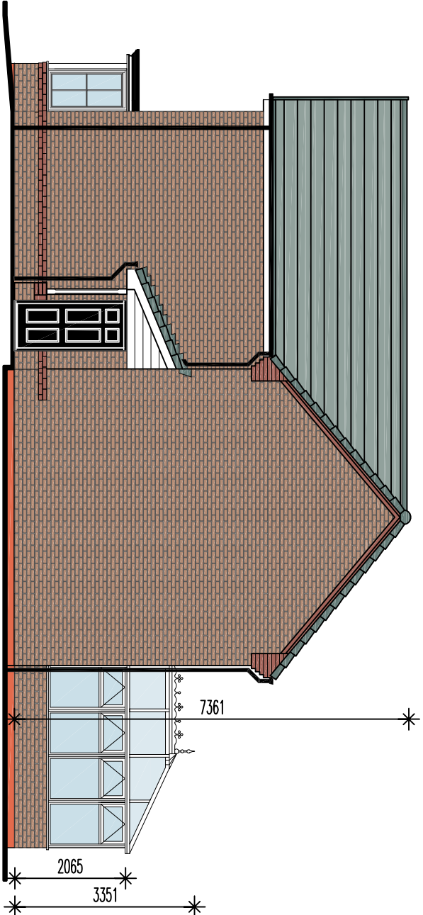
side elevation - with conservatory option
