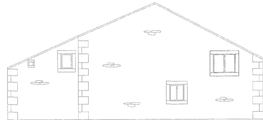
Southeast Elevation
