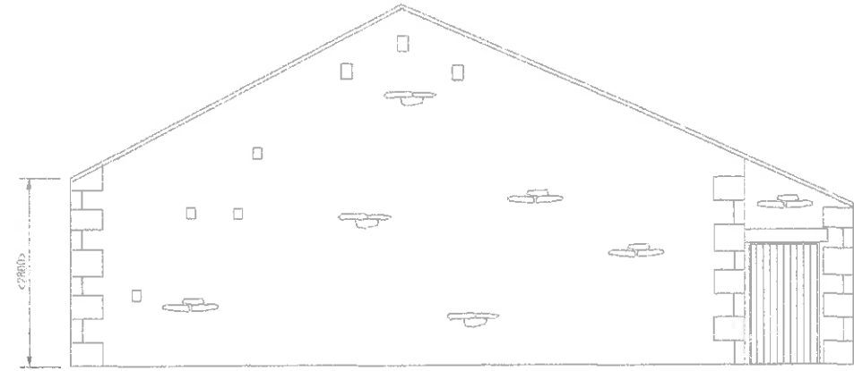
Northwest Elevation
