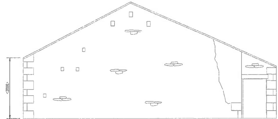
Northwest Elevation
