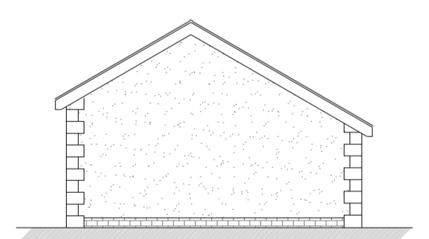
4 Proposed Elevation (1:100)
