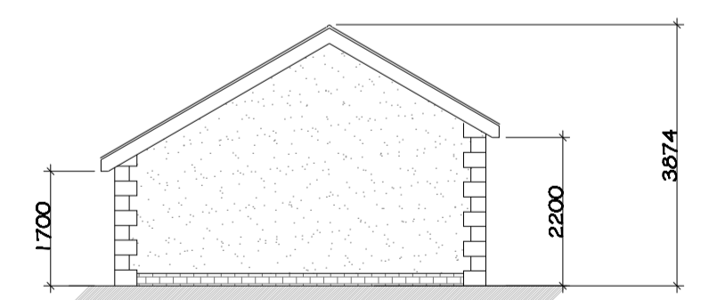
2 Proposed Elevation 1:100
