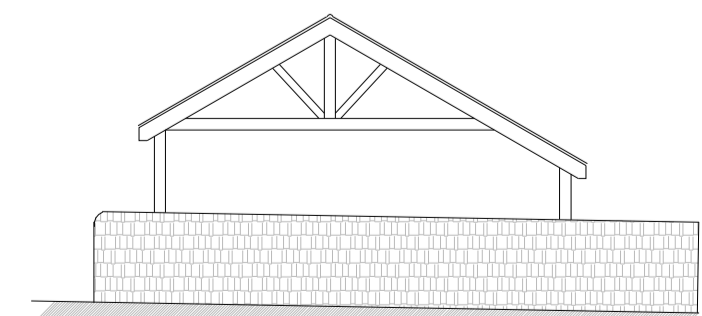
5 Proposed Street Elevation (1:100)
