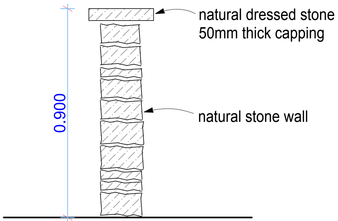
Dwarf wall forming bedroom gardens Scale 1-10
