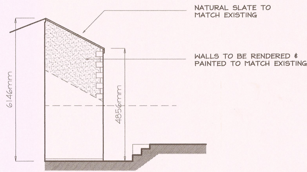
side elevation
