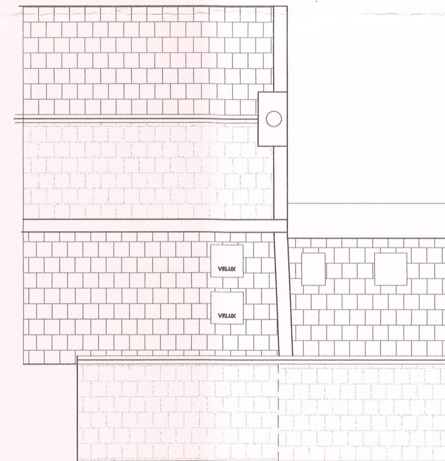
roof plan
