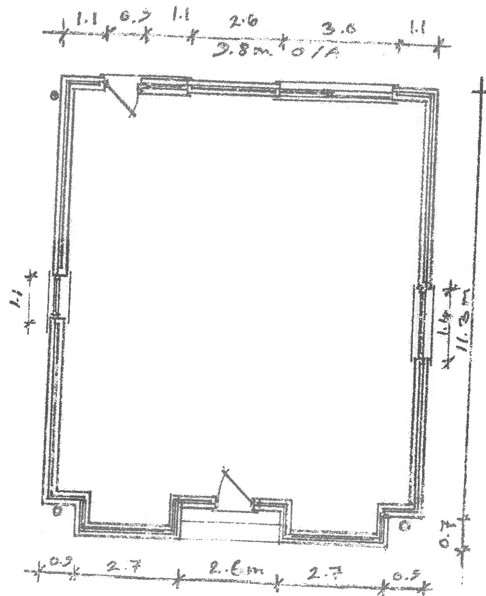
GROUND FLOOR - EXISTING
