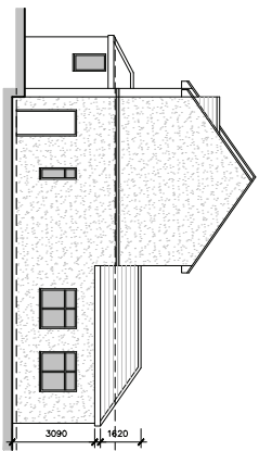
PROPOSED SIDE ELEVATION 1:100
