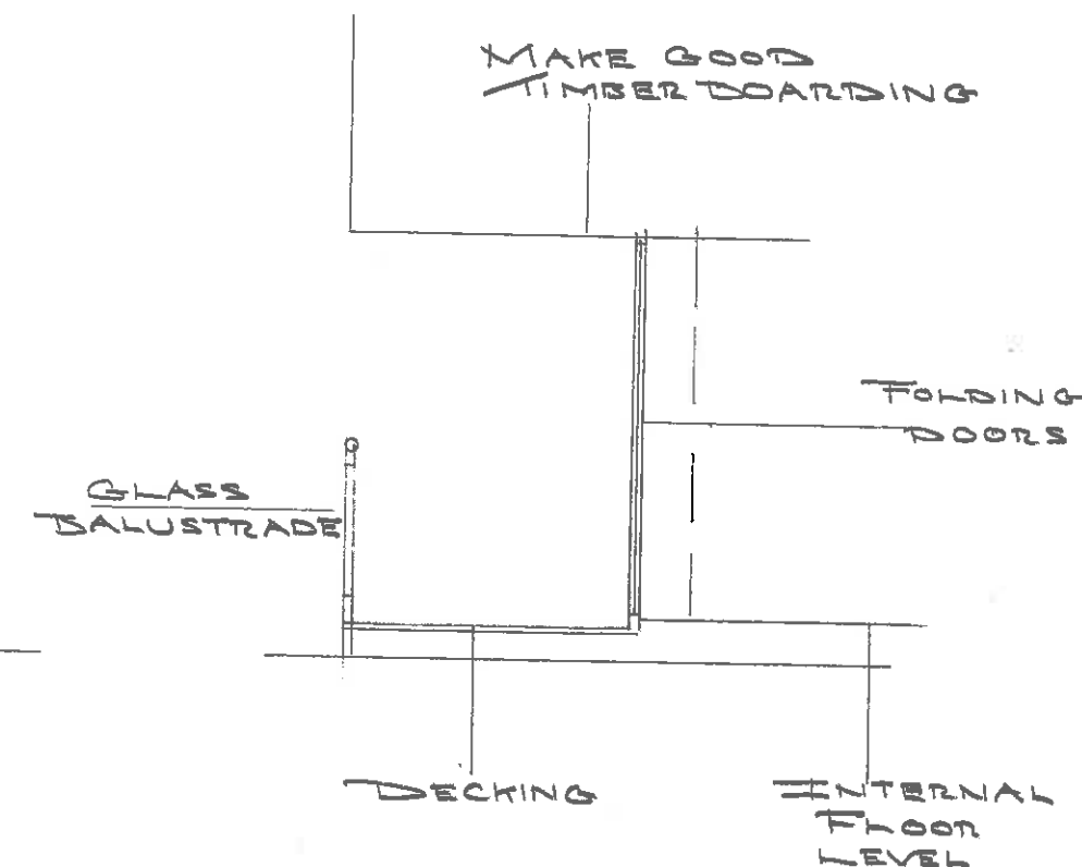
GROUND LEVEL PROPOSED ELEVATION
