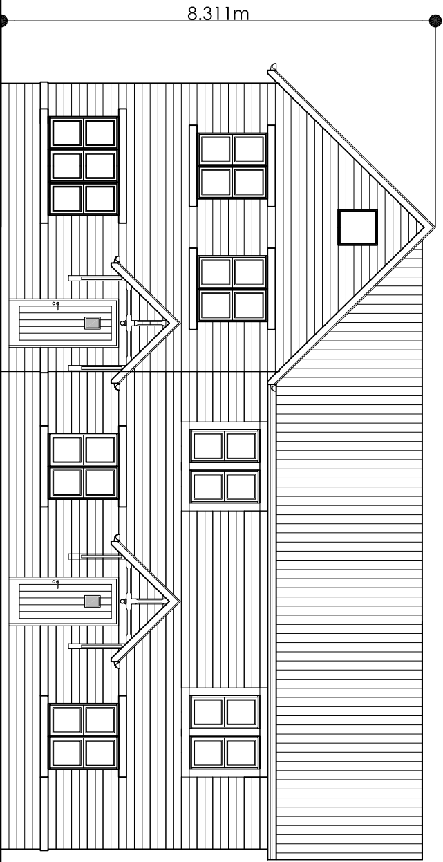
FRONT ELEVATION
