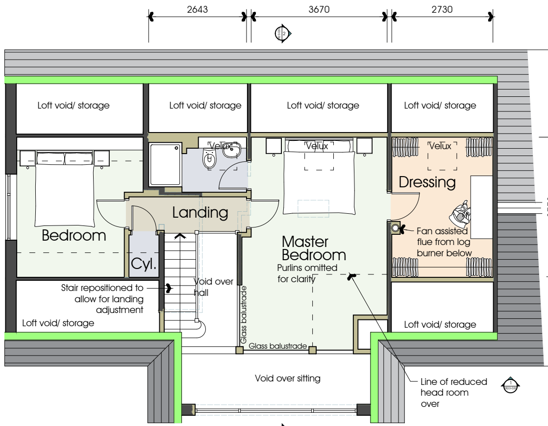
1FL Plan
