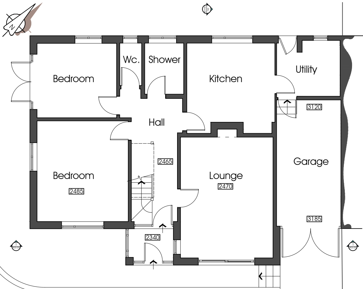
GFL Plan
