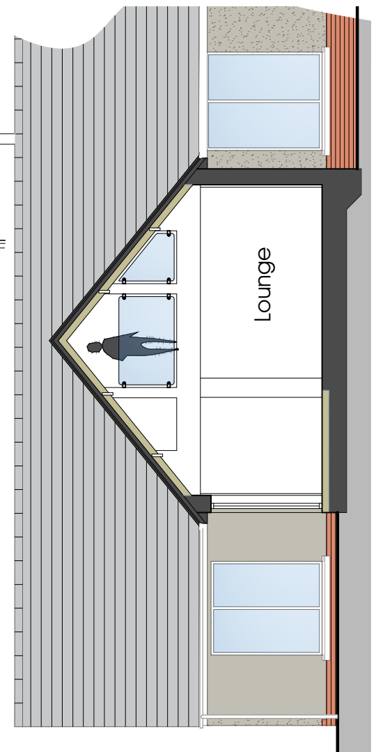
Section 1
