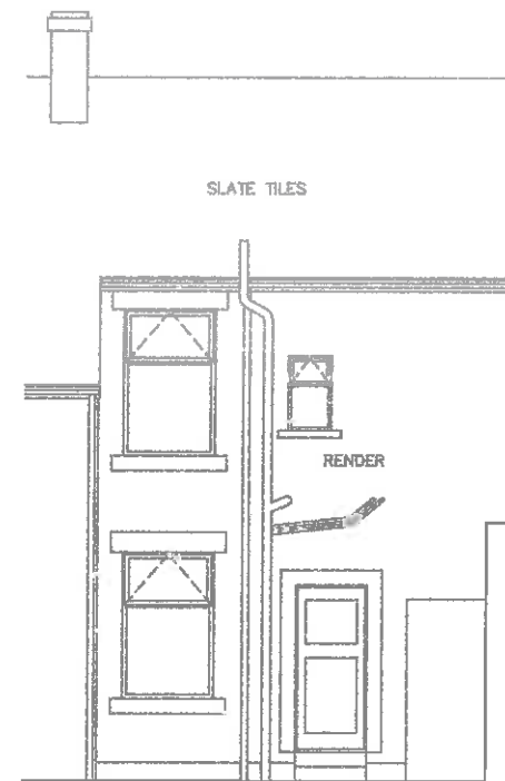
REAR ELEVATION
