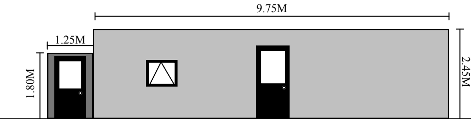
SOUTH ELEVATION
