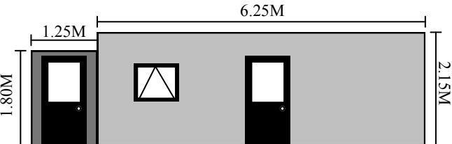
SOUTH ELEVATION
