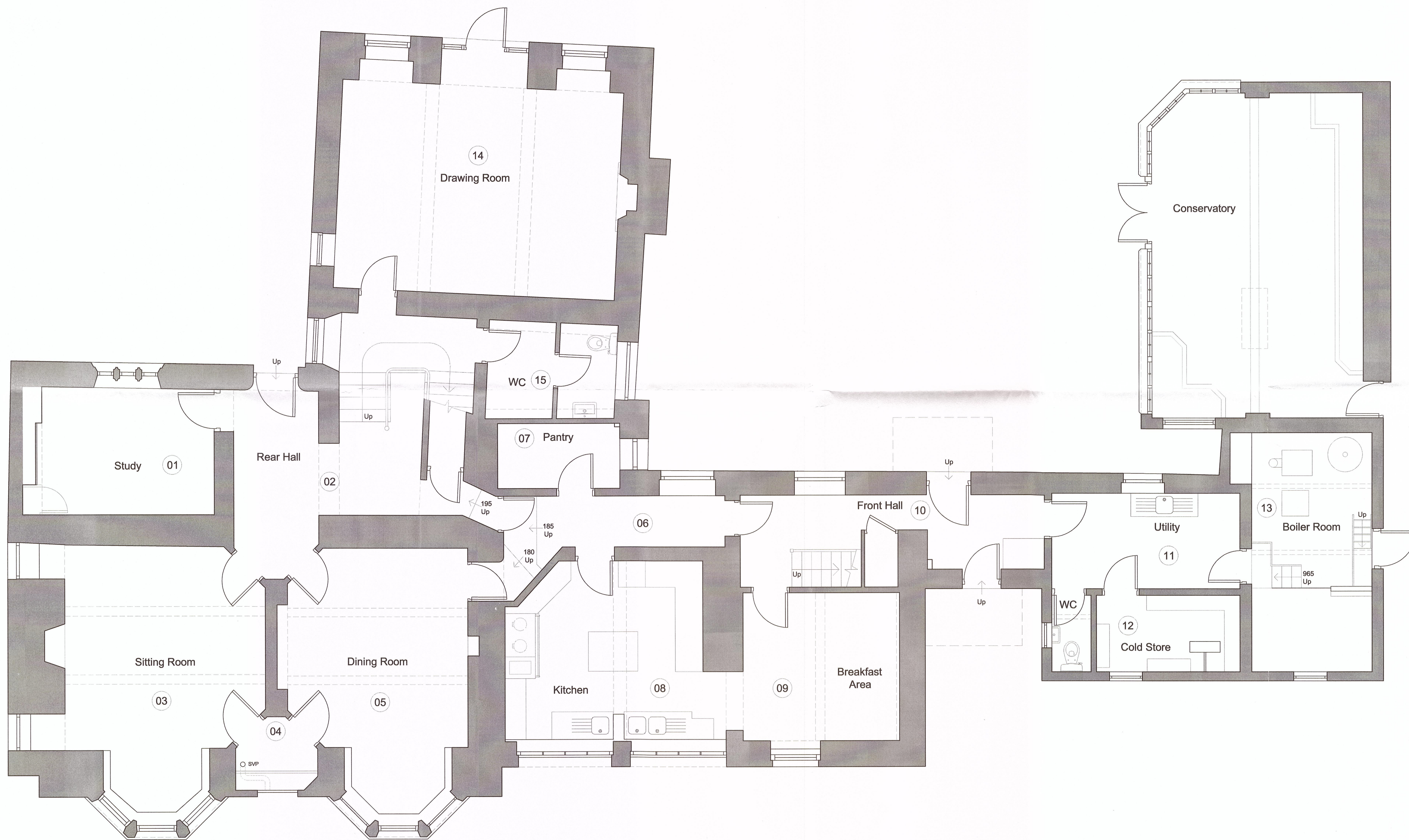
Ground Floor Plan 1:50 Scale
