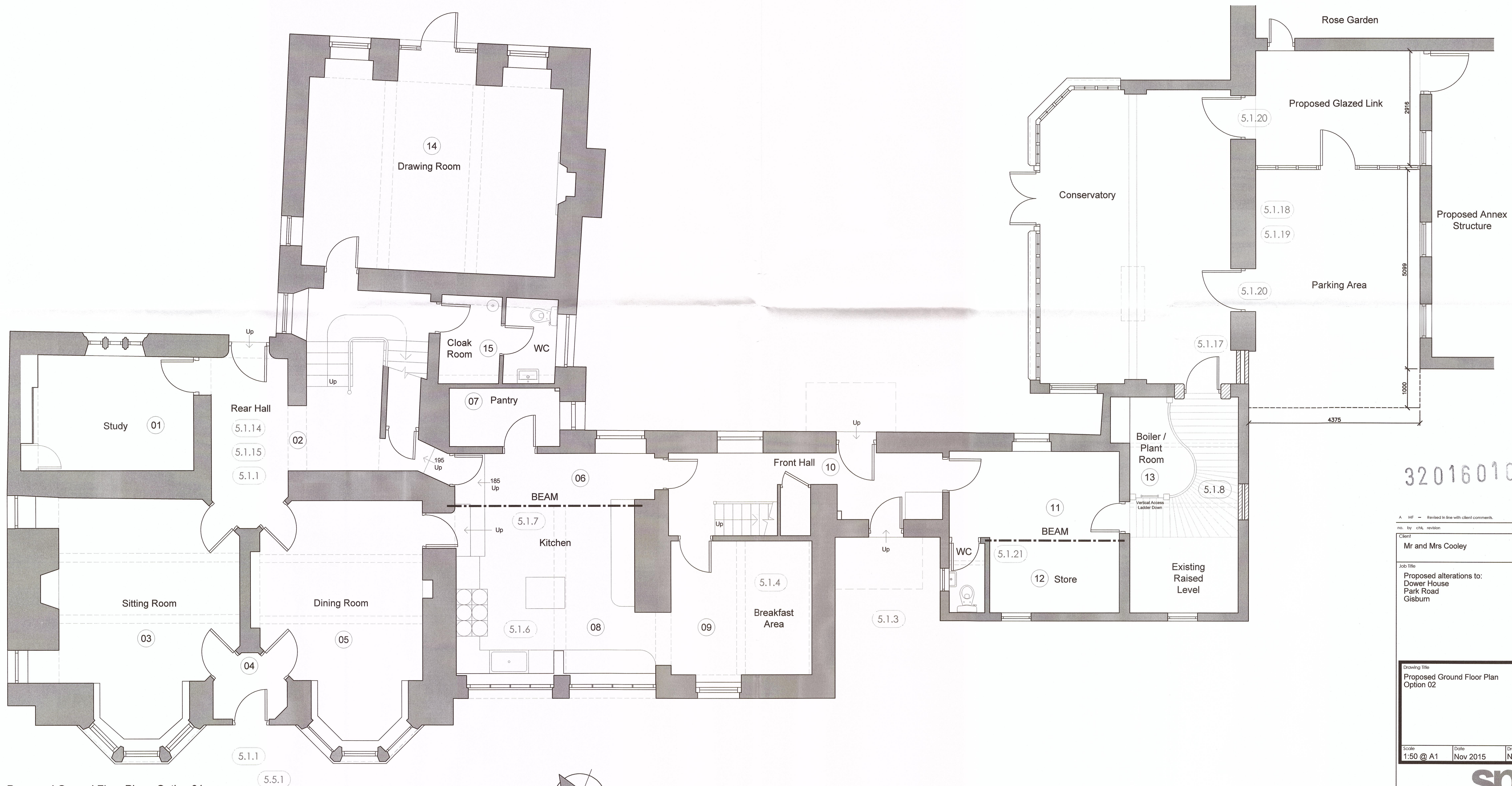
Proposed Ground Floor Plan - Option 01 1:50 Scale
