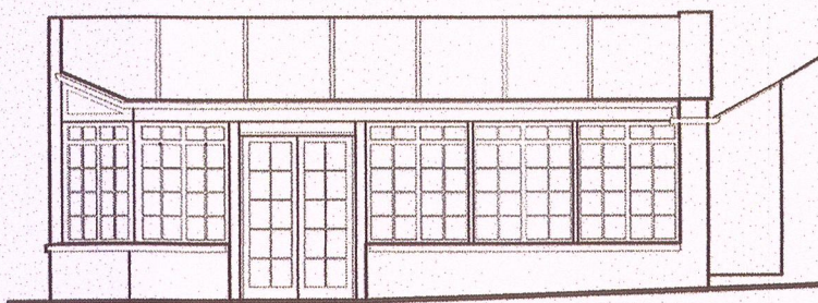
North (Courtyard) Elevation 1:100 Scale
