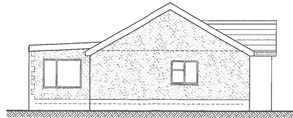
SIDE ELEVATION AS EXISTING SCALE 1:100
