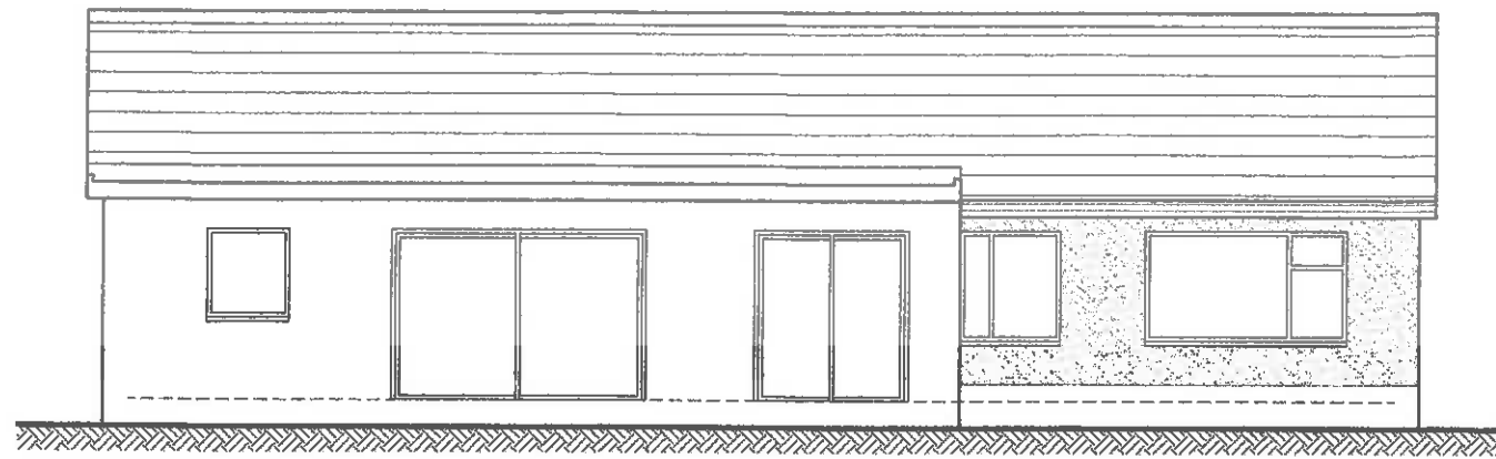
REAR ELEVATION AS EXISTING SCALE 1:100
