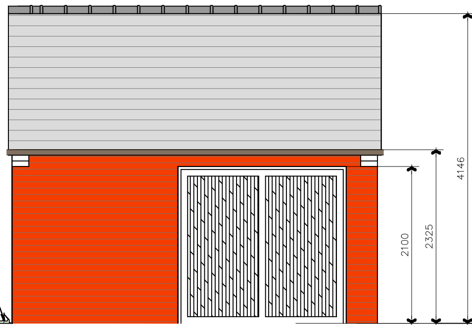
4885 FRONT ELEVATION
