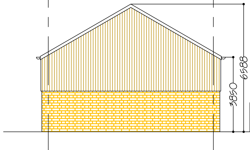
NORTH ELEVATION
