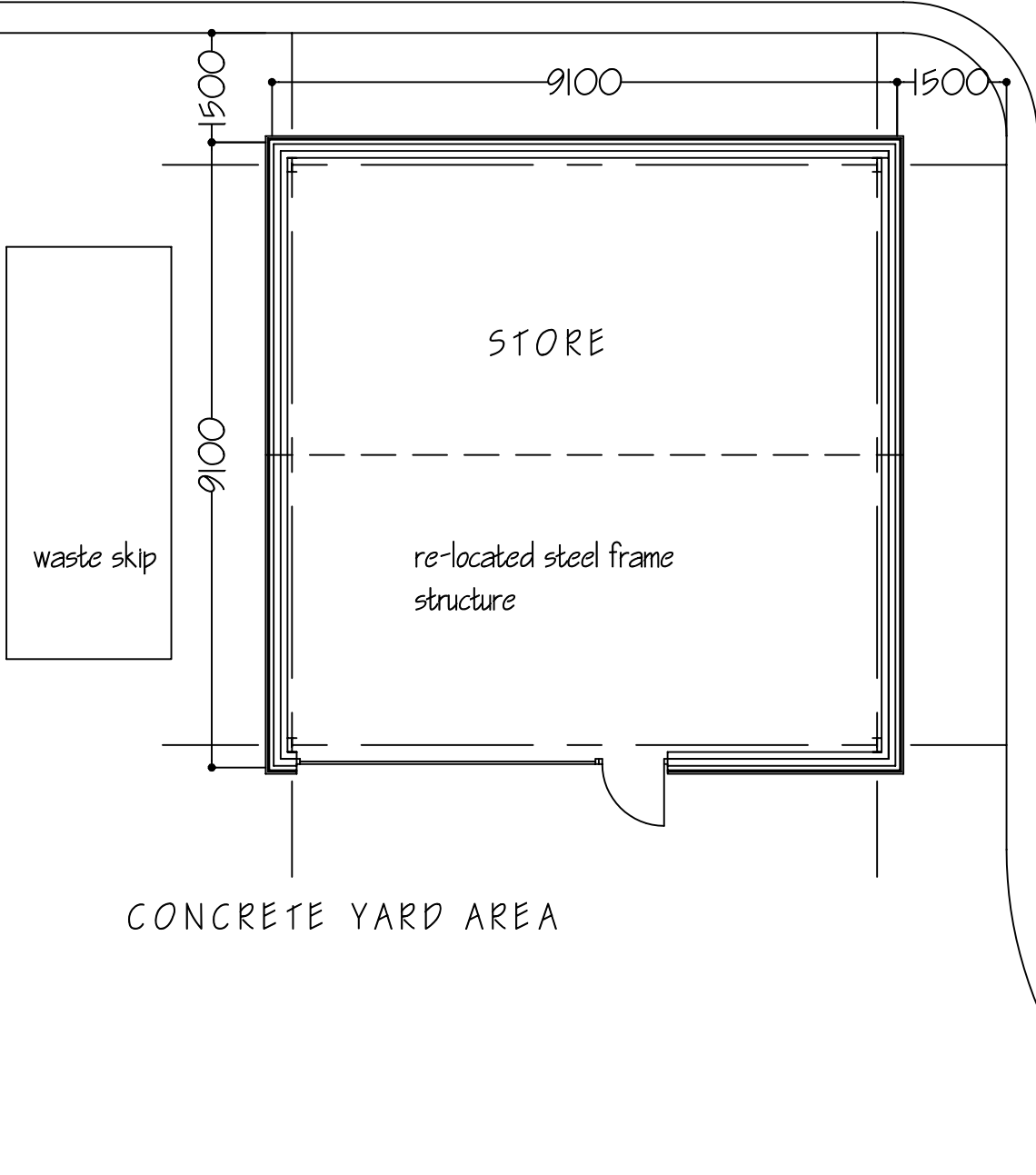
FLOOR LAYOUT 1:100 @ A2 size
