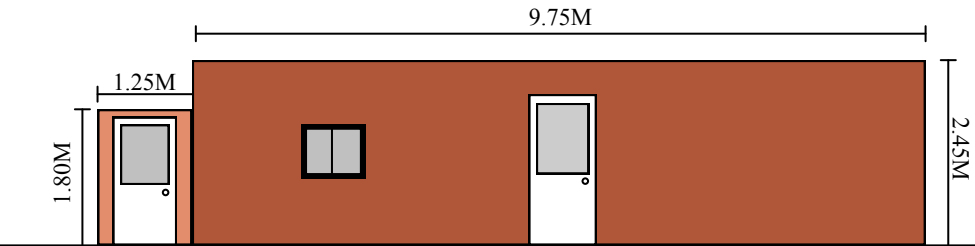
SOUTH ELEVATION
