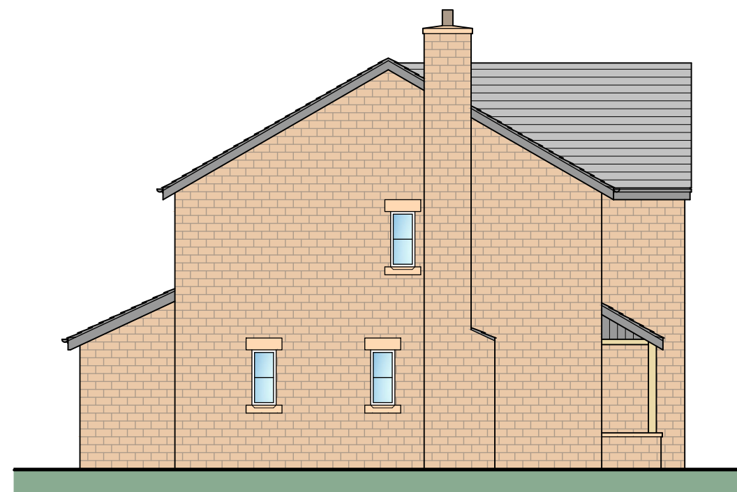
Side Elevation
