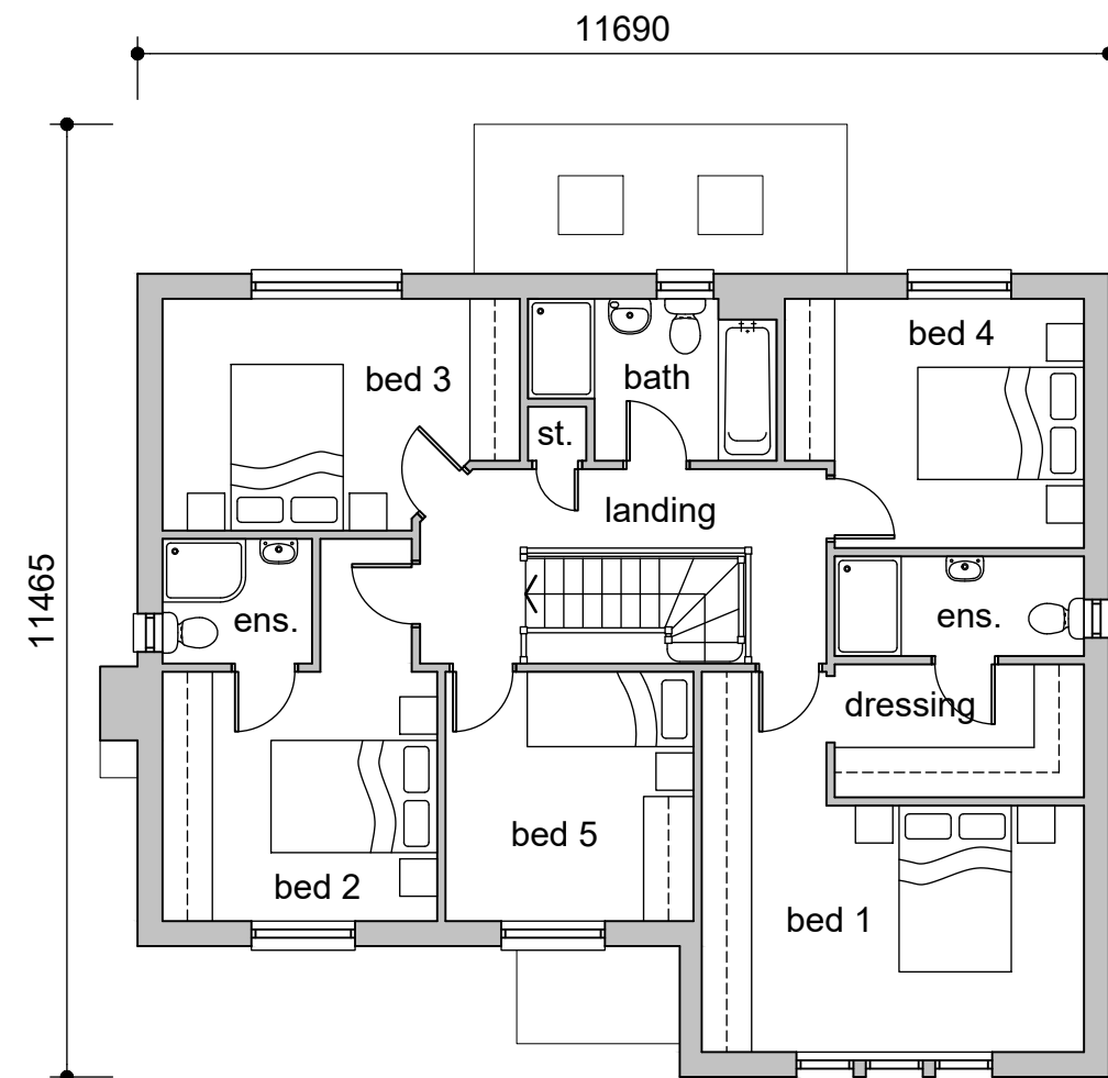
First Floor Plan - 89.2sq.m
