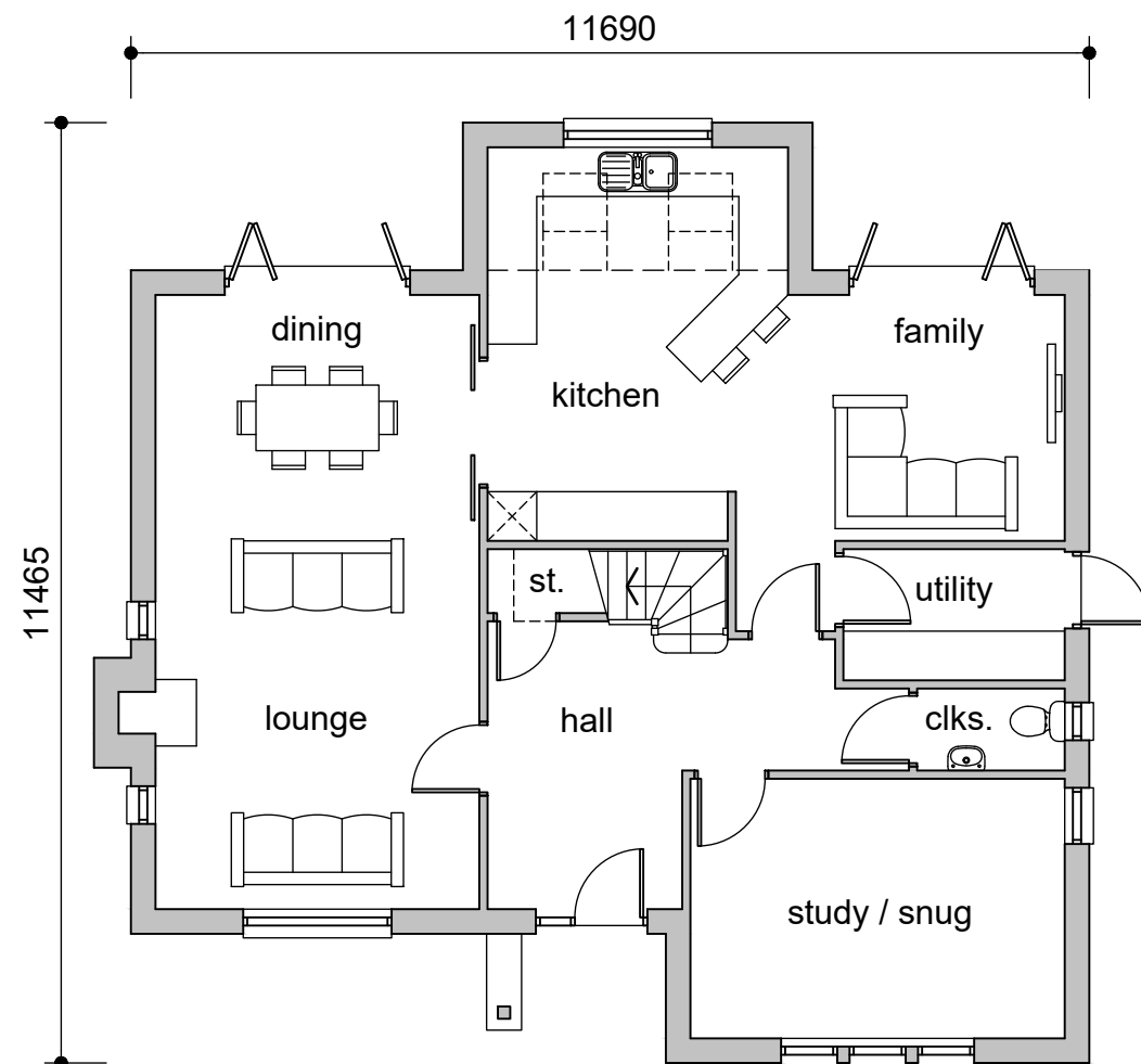
Ground Floor Plan - 96.2sq.m Plot 1 (2 handed)
