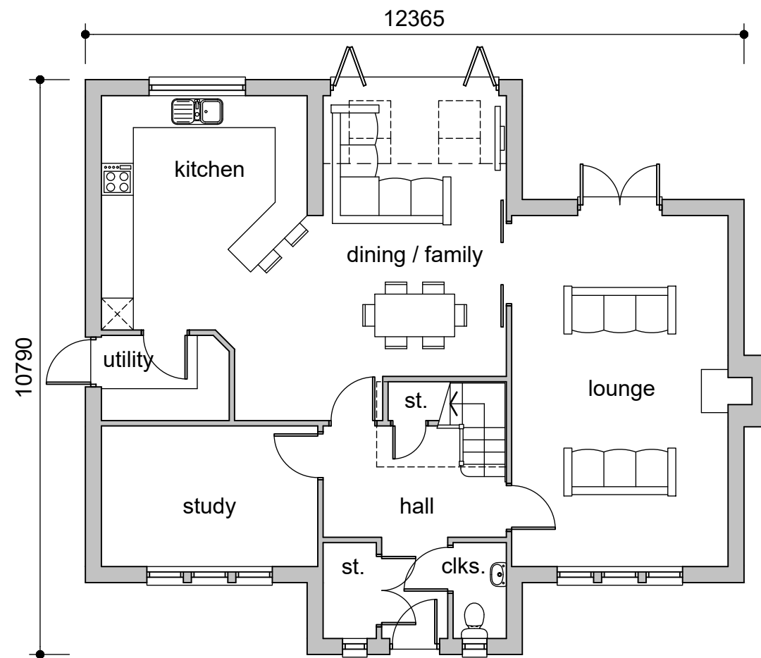
Ground Floor Plan - 98.2sq.m Plot 3 + 9 (6 handed)
