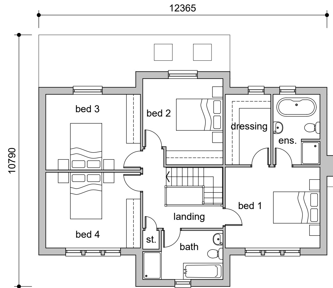
First Floor Plan - 83.5sq.m
