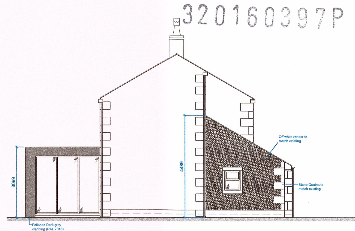
Proposed Side Elevation (West facing stables)
