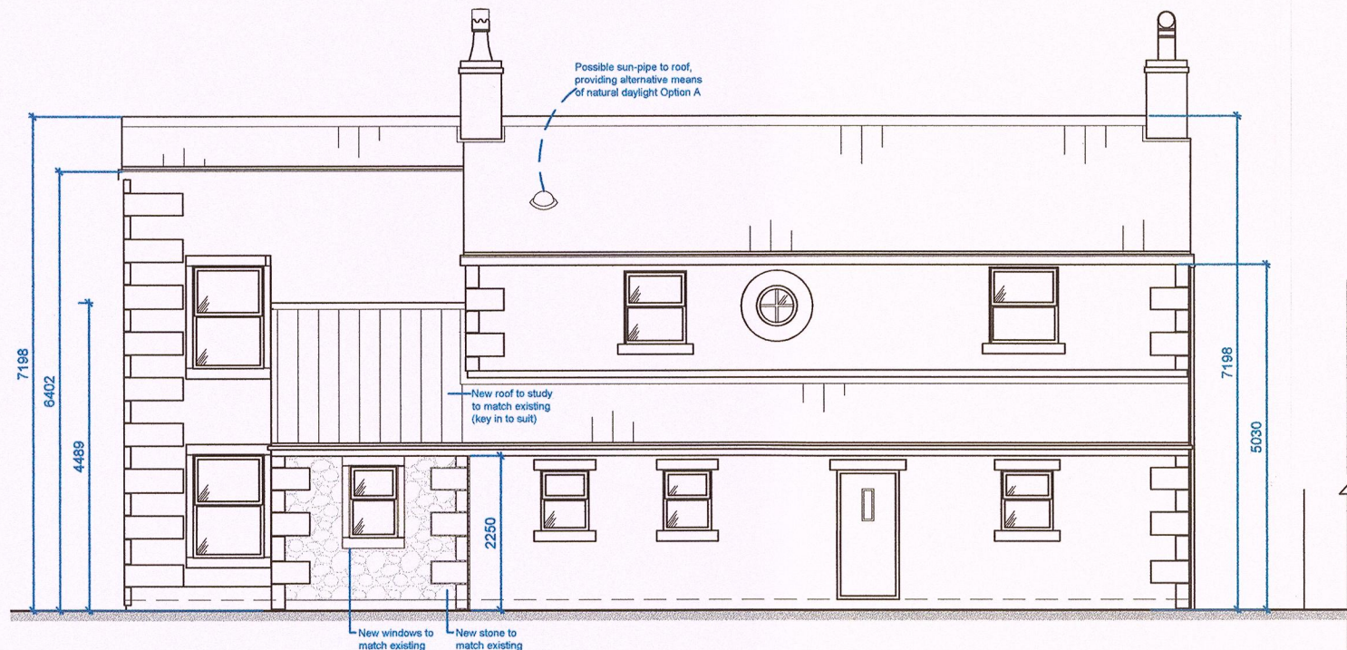
Proposed Front Elevation (North facing over driveway)
