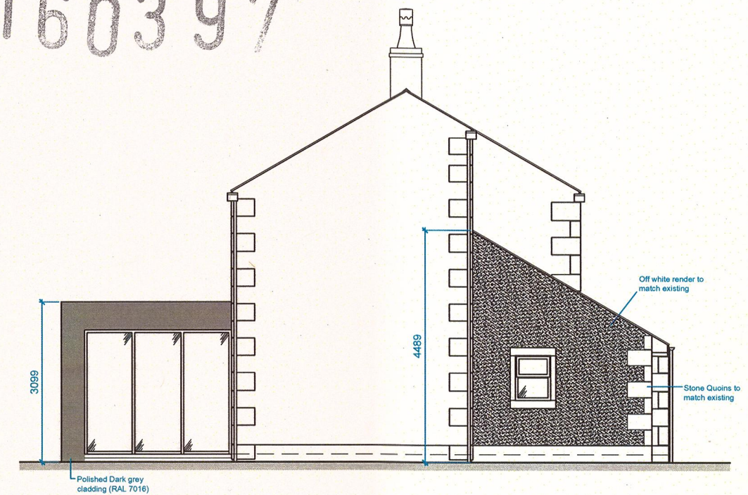
Proposed Side Elevation (West facing stables)
