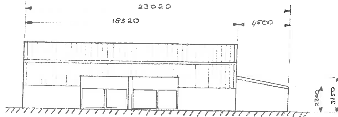
ELEVATION LOOKING WEST
