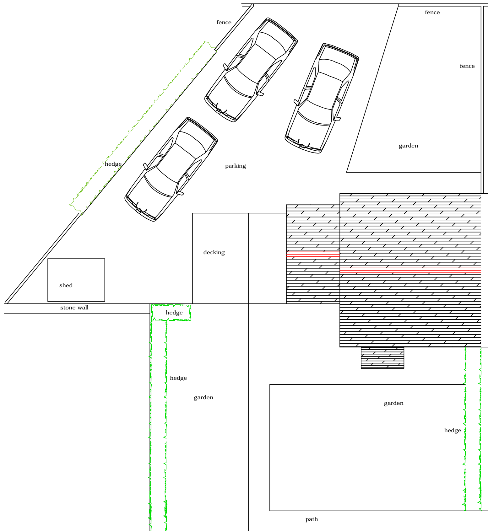
EXISTING SITE PLAN scale 1:100
