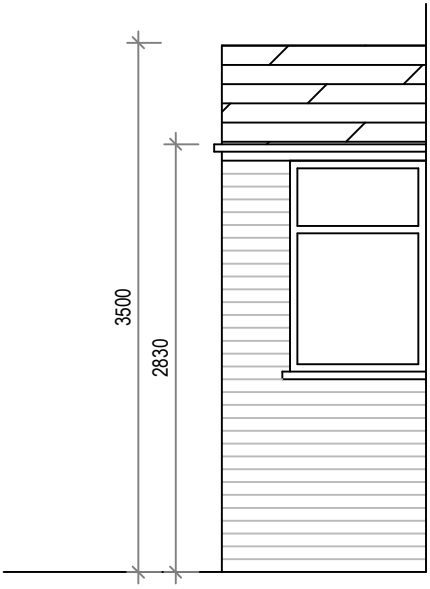
PROPOSED SIDE ELEVATION TO PORCH
