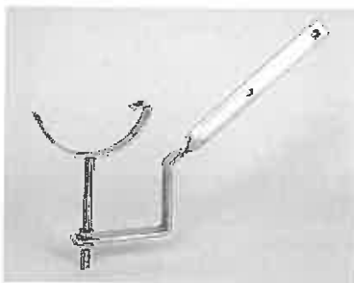
'drive-in' galvanised gutter bracket, with half round Aluminium gutters powder coated balck, by Alumasc or equal approved
