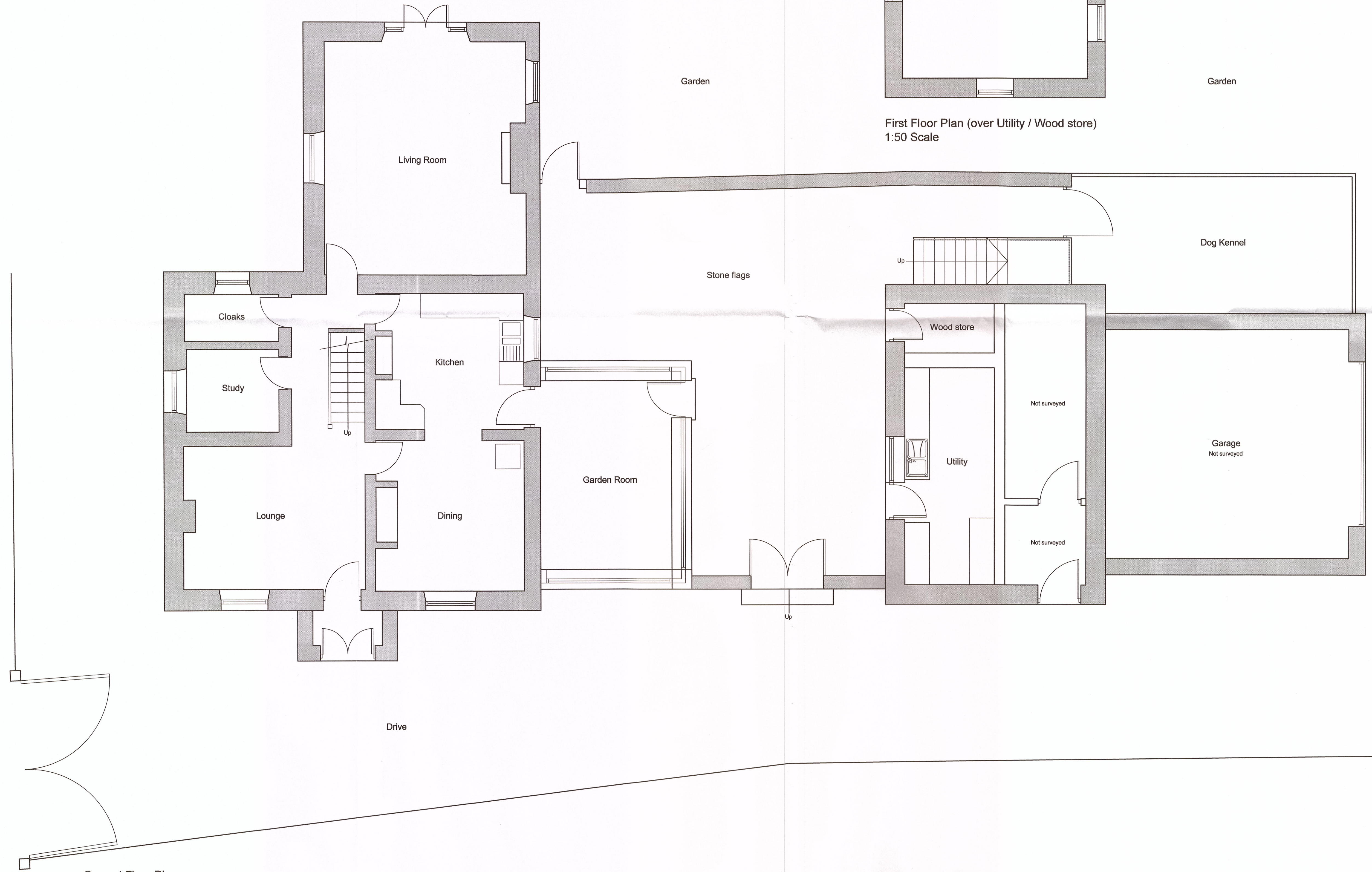
Ground Floor Plan 1:50 Scale
