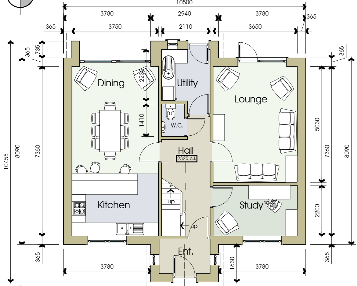
Ground scale 1:100
