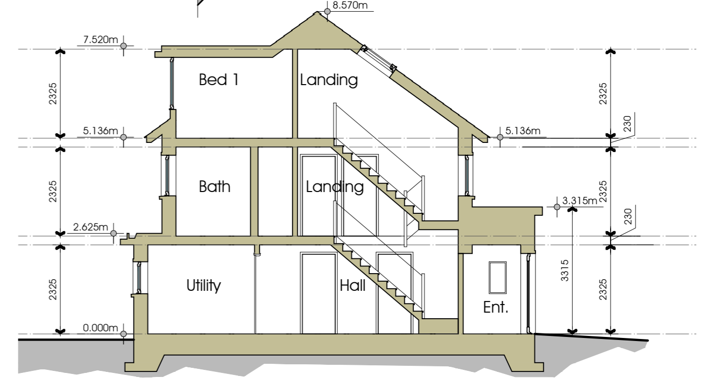
Section scale 1:100
