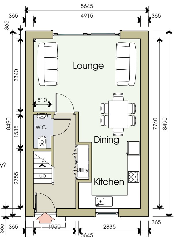
Ground scale 1:100
