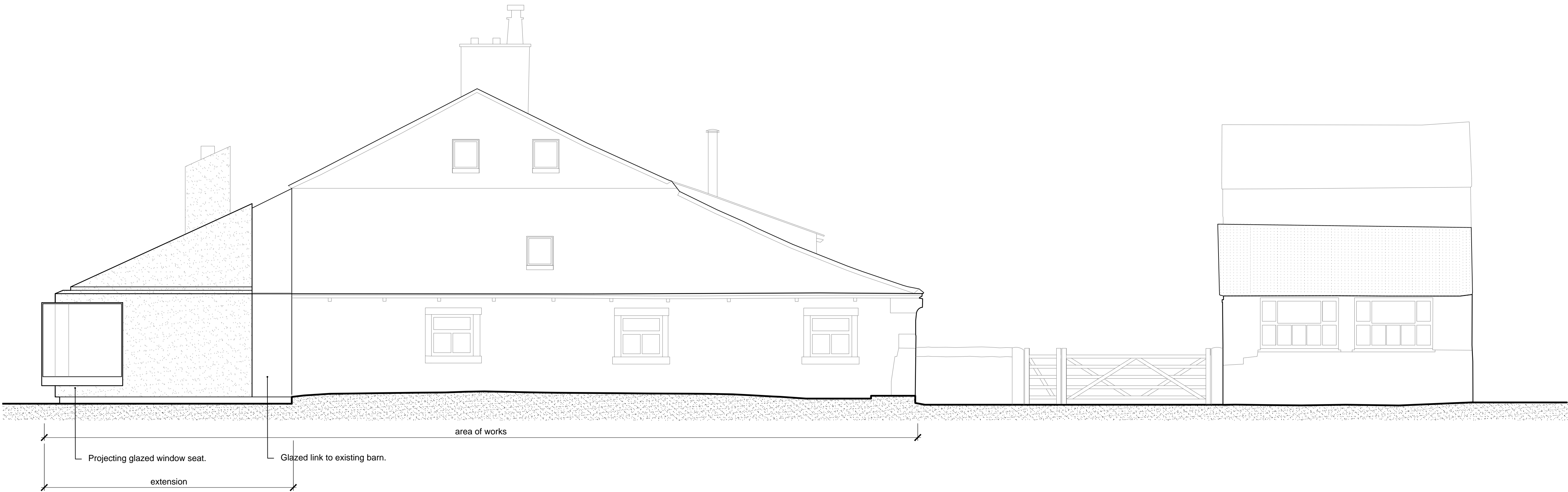
North Elevation
