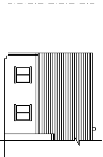
ELEVATION A EXISTING ELEVATIONS @1:200
