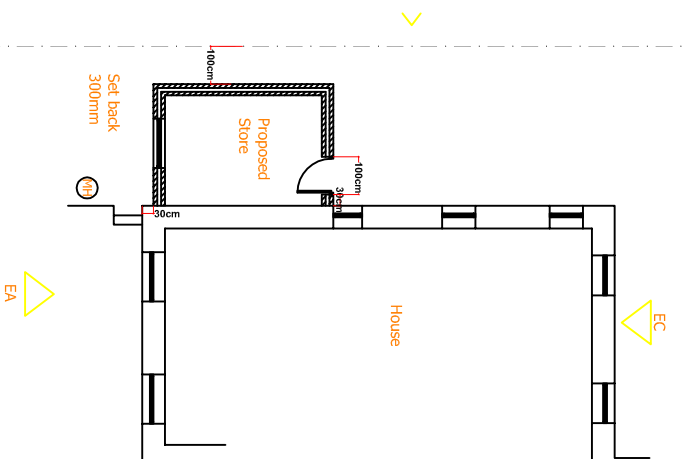
PROPOSED GROUND FLOOR PART PLAN @1:200
