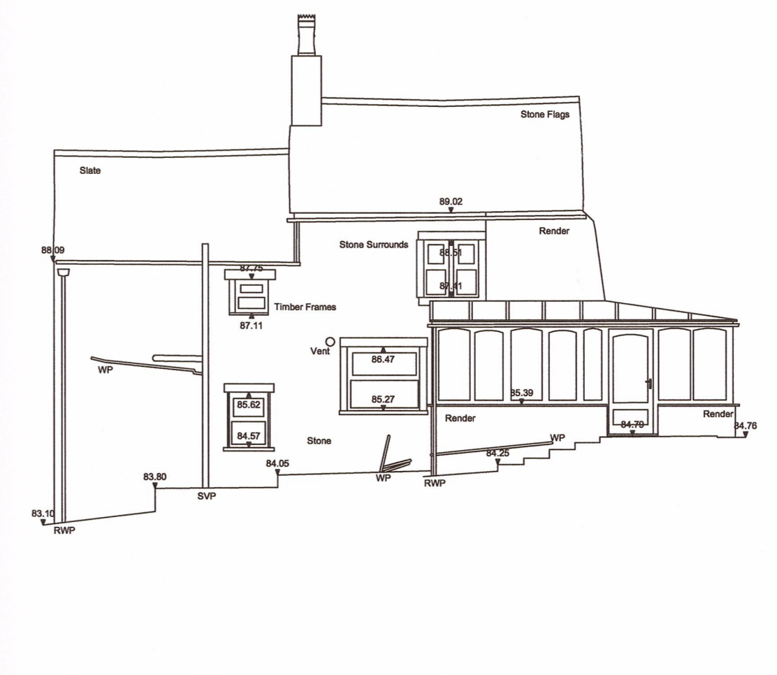
North Elevation ▼ 80.00m above OS Datum
