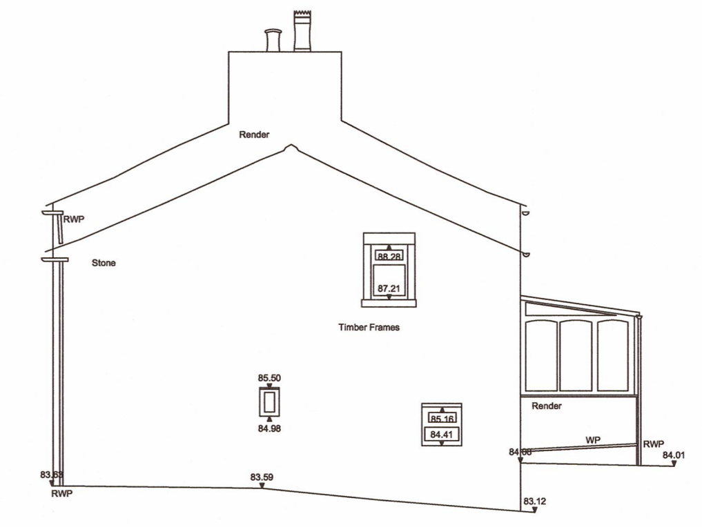
East Elevation ▼ 80.00m above OS Datum
