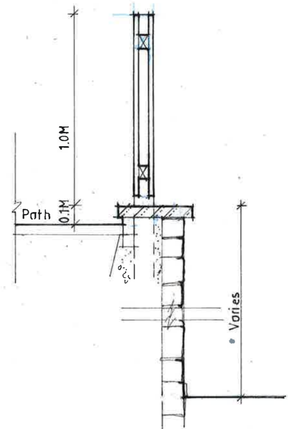
SECTION
