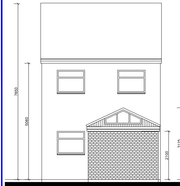
Rear Elevation
